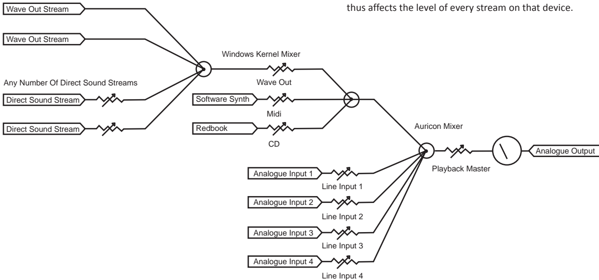
Fig 1-3 Output Mixing
