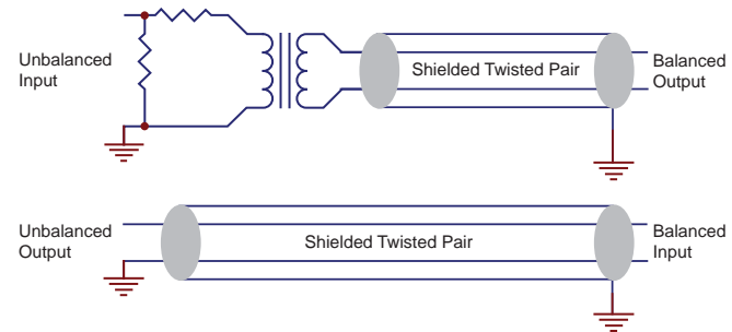
Fig 1-1: Connecting the Auricon 4.4 to Unbalanced Inputs and Outputs
