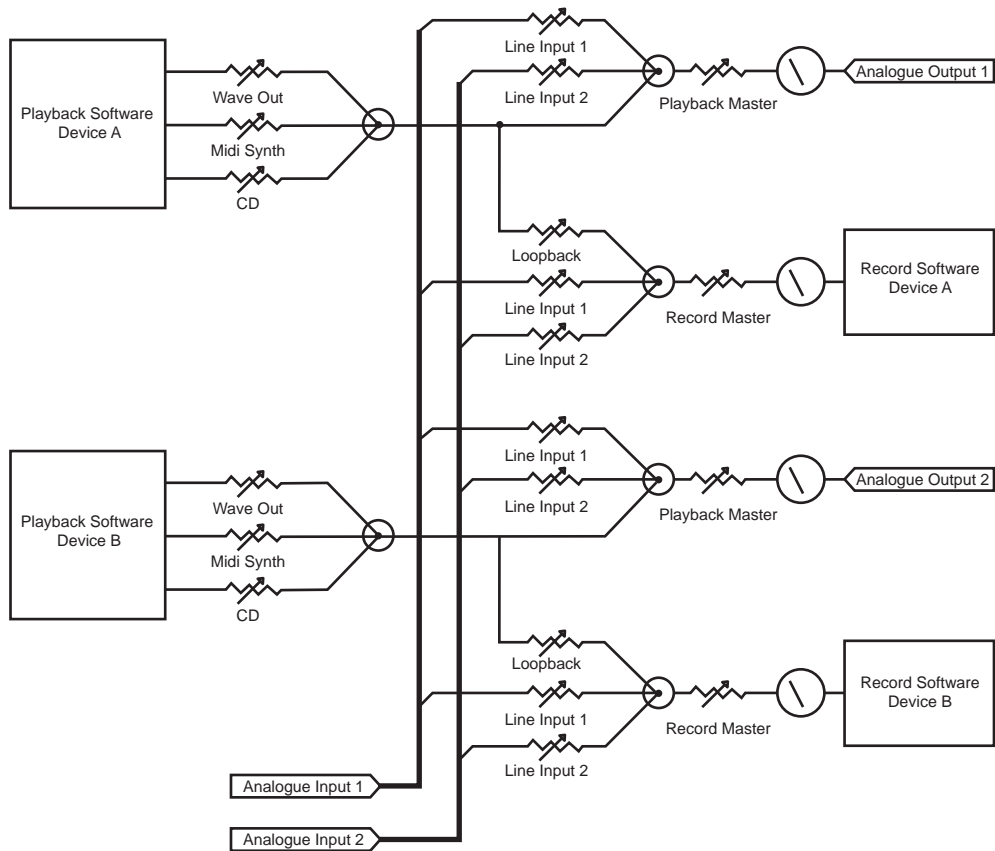
Fig 1-2 Auricon 4.4 Topology
