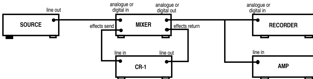
2. CR-1 SERIES 2 used on the effects loop within a studio environment.
