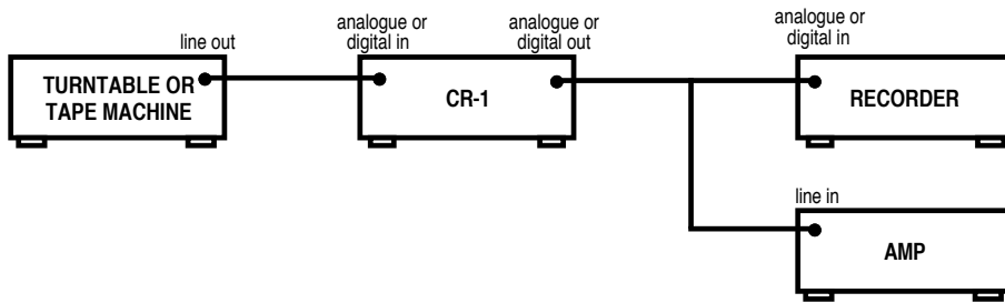
1. CR-1 SERIES 2 used in-line for transcription or broadcast purposes.
