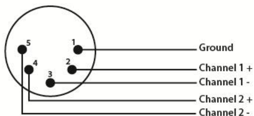
5-Pin Male XLR (rear view)
