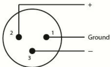
3-Pin Male XLR (rear view)
