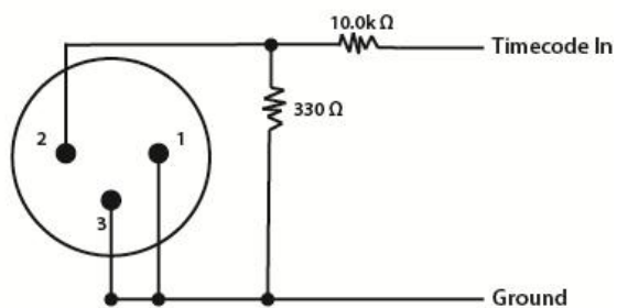
3-Pin Male XLR (rear view)
